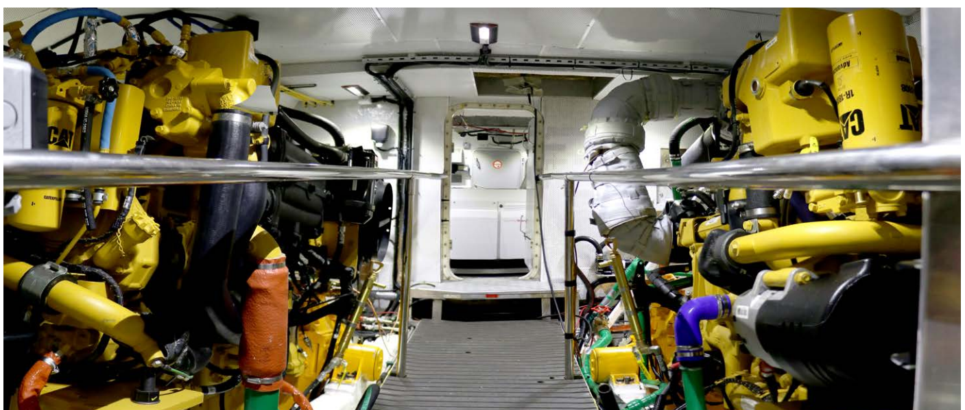
Installation of twin Caterpillar C18 810HP Engines to a 60' Stretched Arun MOD Police Patrol Boat
